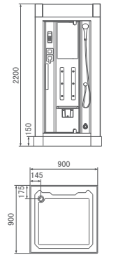
MODEL:WS-502 SIZE:900 × 900 × 2200mm
