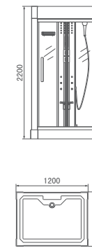
MODEL:WS-500 SIZE:1200 × 900 × 2200mm
