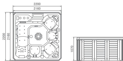
MODEL:WS-S01(TV) SIZE:2200 × 2200 × 1070mm
