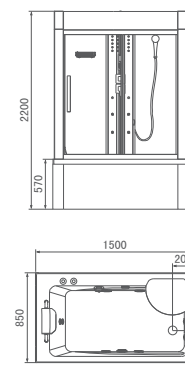
MODEL:WS-501 SIZE:1500 × 850 × 2200mm
