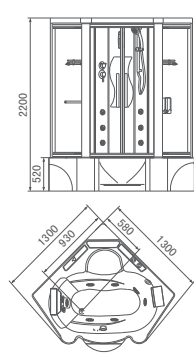
MODEL:WS-609P SIZE:1300 × 1300 × 2200mm
