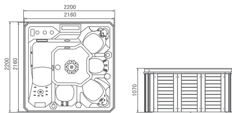
MODEL:WS-S01A SIZE:2200 × 2200 × 1070mm
