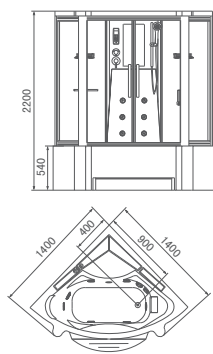
MODEL:WS-600P SIZE:1400 × 1400 × 2200mm
