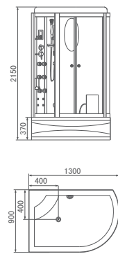
MODEL:WS-903R(Left/Right) SIZE:1300 × 900 × 2150mm
