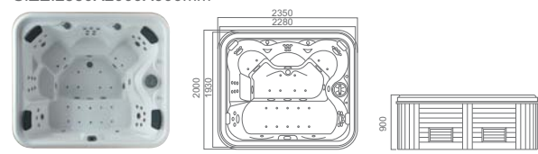
2. MODEL:WS-093A SIZE:2350X2000X900mm
