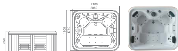
1. MODEL:WS-094A SIZE:2100X1800X850mm
