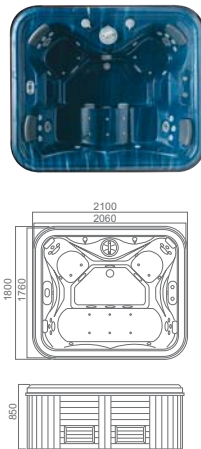
3. MODEL:WS-094B SIZE:2100X1800X850mm
